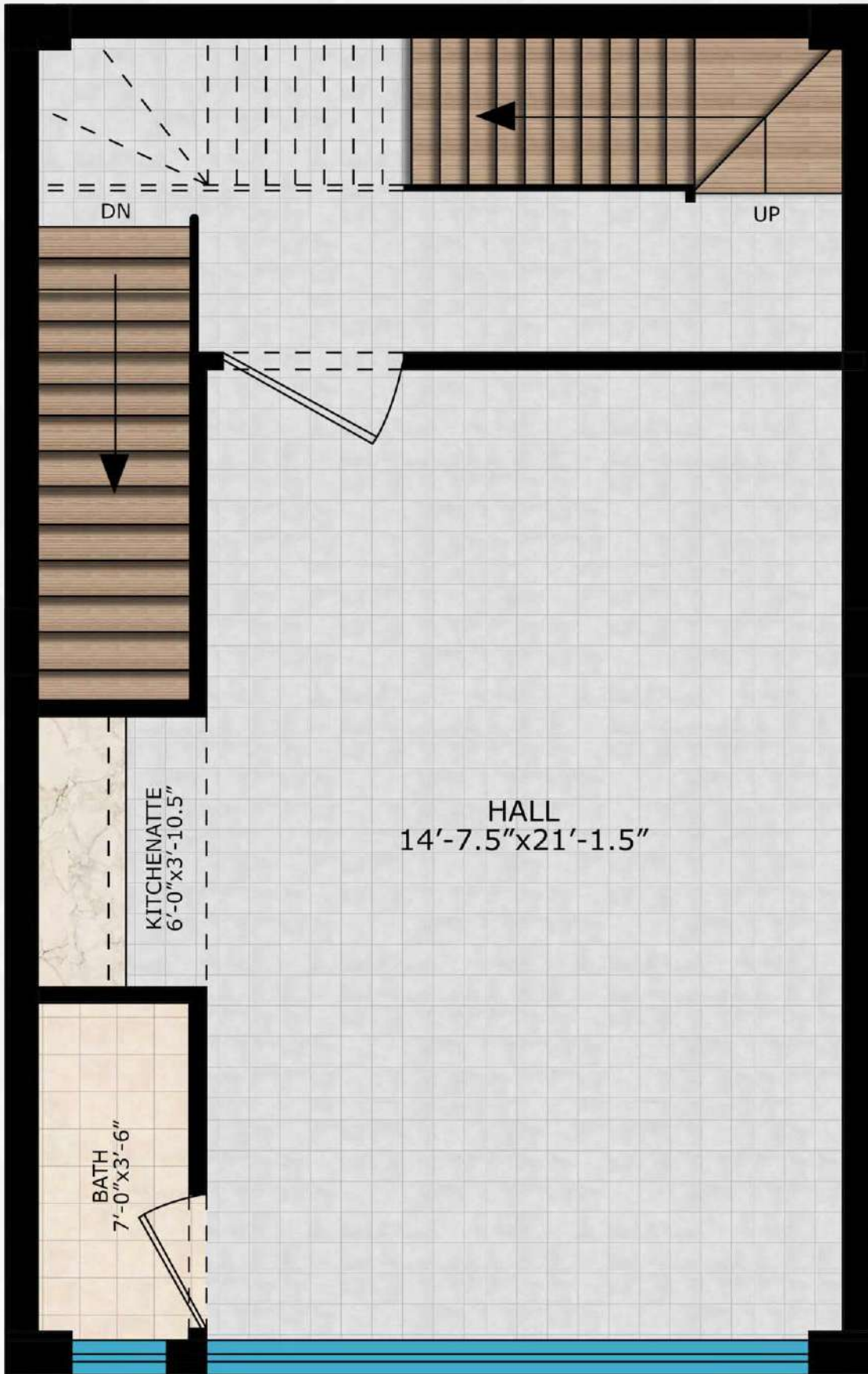
FIRST FLOOR
